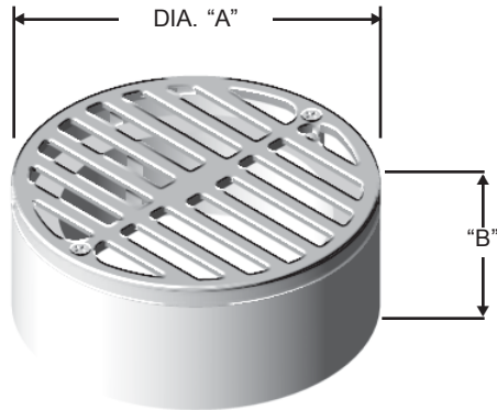
3" & 4" Round Brass Grate
