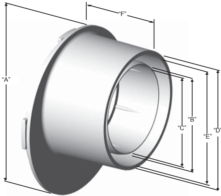
Universal Offset Outlet
